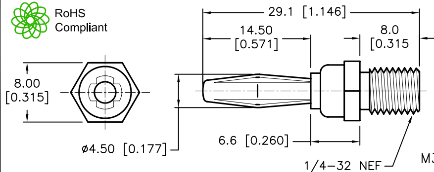
PLUG BODY
