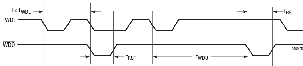
WATCHDOG TIMING ( \overline{W}/T = LOW), WINDOW MODE
