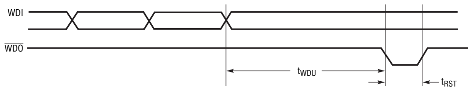
WATCHDOG TIMING ( \overline{W}/T = HIGH), TIMEOUT MODE
