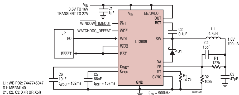
1.8V Step-Down Converter with System Reset Generated by Watchdog Timing or Output Voltage Failure
