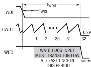
(13b) \overline{W}/T = \text{Low} . Subsequent Negative Edges Must Occur Within a Fixed Time Window
