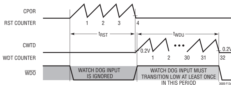
(13c) \overline{W}/T = \text{Low} . Restart Sequence After a Timing Fault
