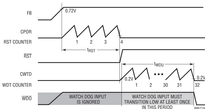
(13a) \overline{W}/T = \text{Low} . The First Valid Negative Edge on WDI Must Occur Before the Watchdog Timer Expires
