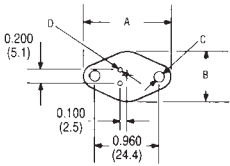
TO-66
