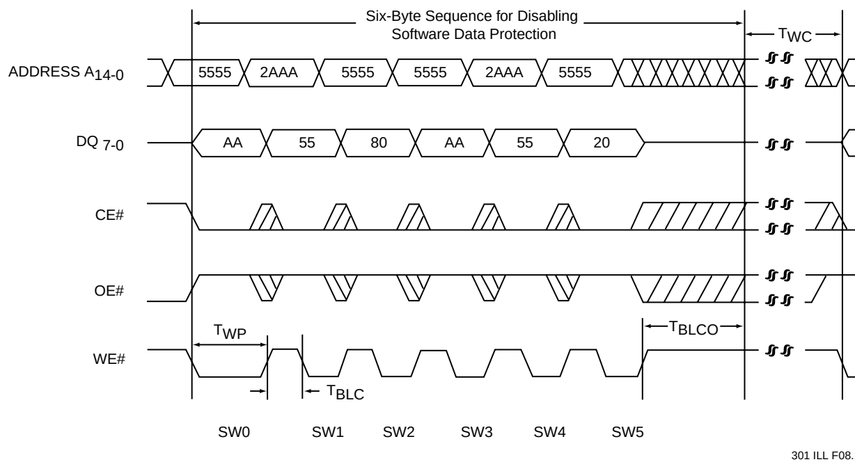
FIGURE 8: SOFTWARE DATA PROTECT DISABLE TIMING DIAGRAM
