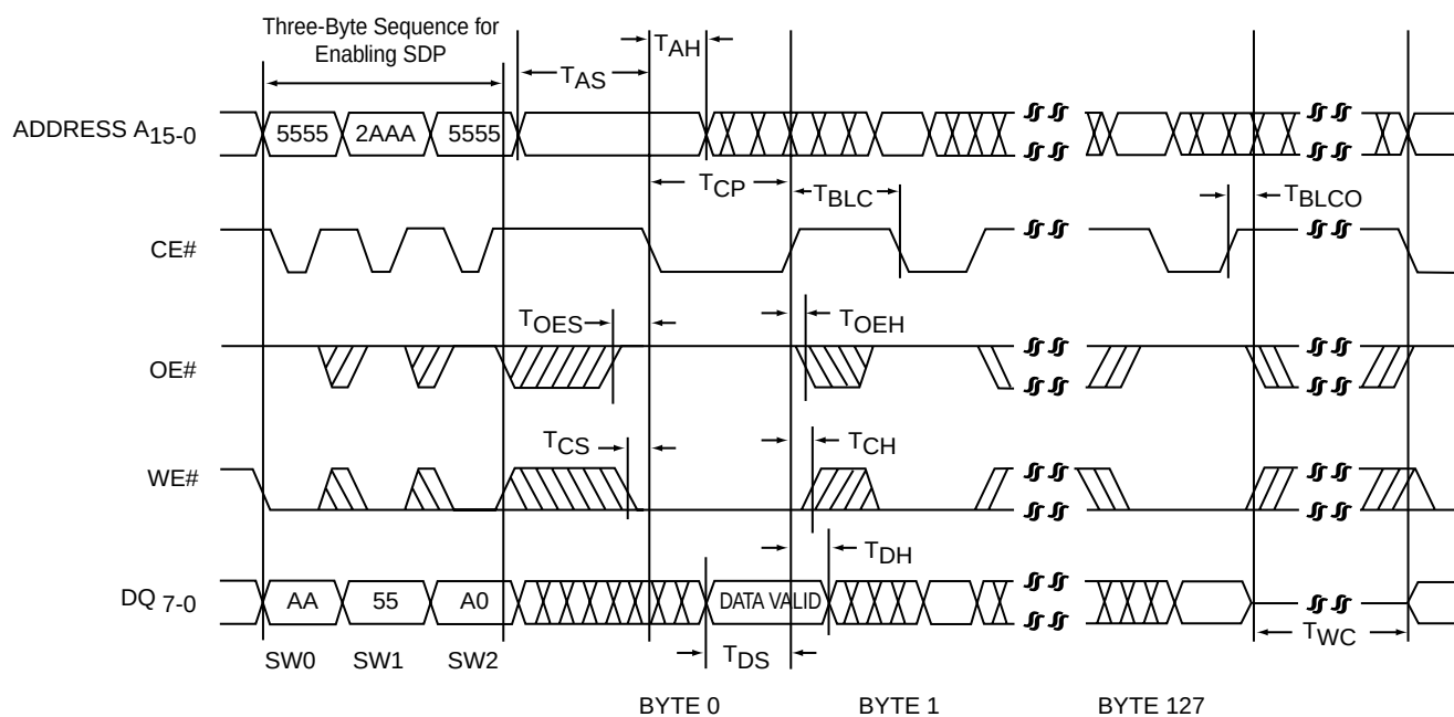
FIGURE 5: CE# CONTROLLED PAGE-WRITE CYCLE TIMING DIAGRAM
