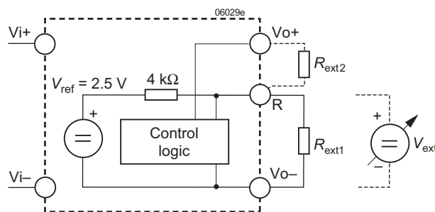
Fig. 15 Output voltage control for single-output models, -0503-models, and double-output models fitted with option R by means of the R input.
