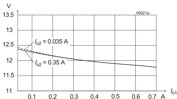
Fig. 11 Cross load regulation V_{o1} versus I_{o1} (typ.) for various I_{o2} (2 x 12 V).
