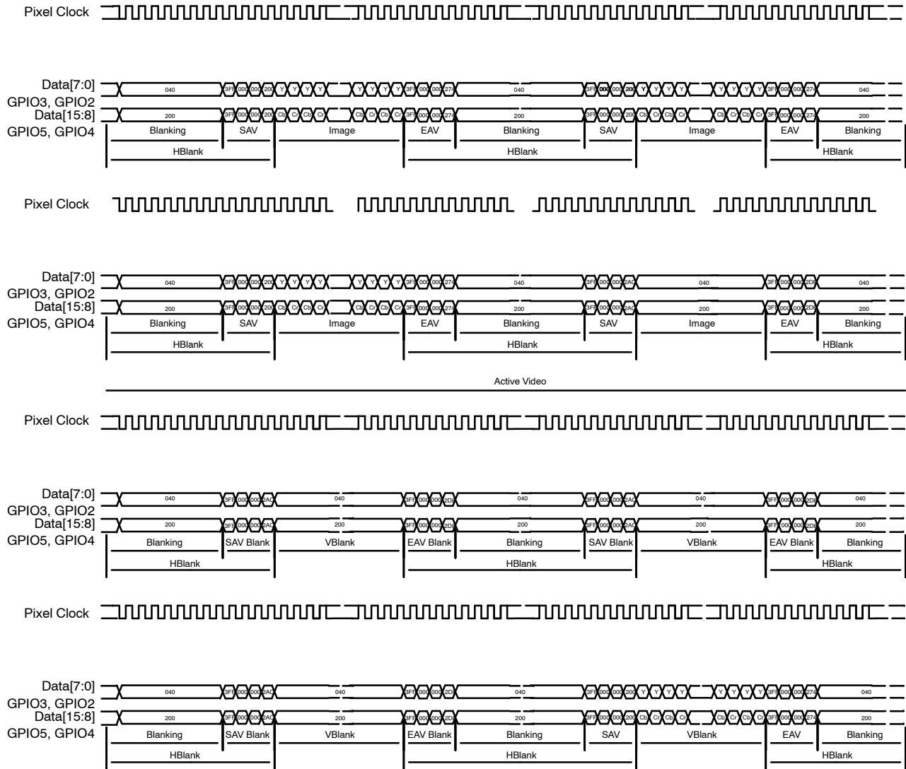
Figure 14. SMPTE296M Output
