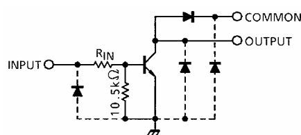
TD62597AFNG R_{IN}=2.7\text{k} TD62598AFNG R_{IN}=10.5\text{k}
