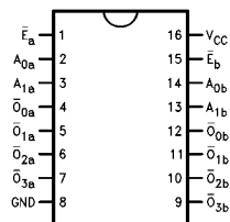
Pin Assignment for DIP and SOIC
