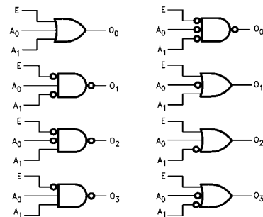
FIGURE 1. Gate Functions (Each Half)
