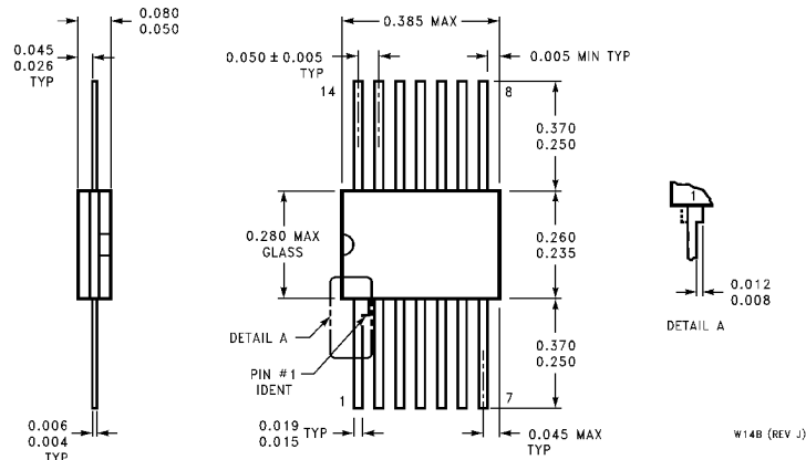
14-Lead Ceramic Flat Package (W) Order Number 54LS20FMB or DM54LS20W Package Number W14B
