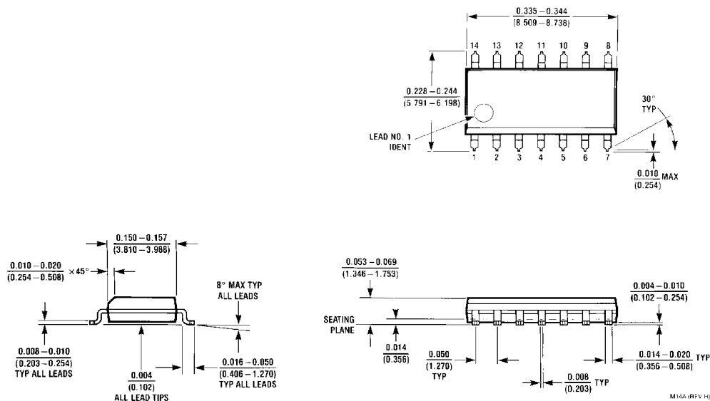
14-Lead Small Outline Molded Package (M) Order Number DM74LS20M Package Number M14A
