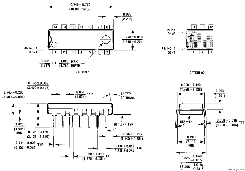
14-Lead Molded Dual-In-Line Package (N) Order Number DM74LS20N Package Number N14A
