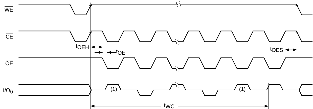
Figure 8. Toggle Bit
