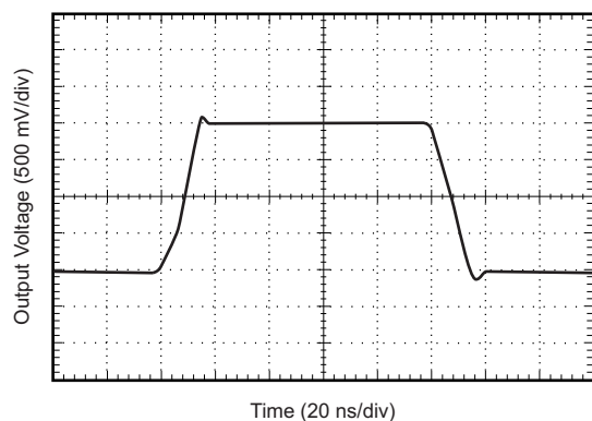
Figure 9. NONINVERTING LARGE-SIGNAL STEP RESPONSE
