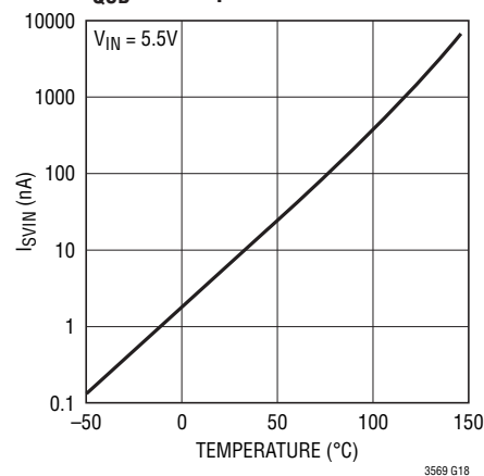
I_{QSD} vs Temperature
