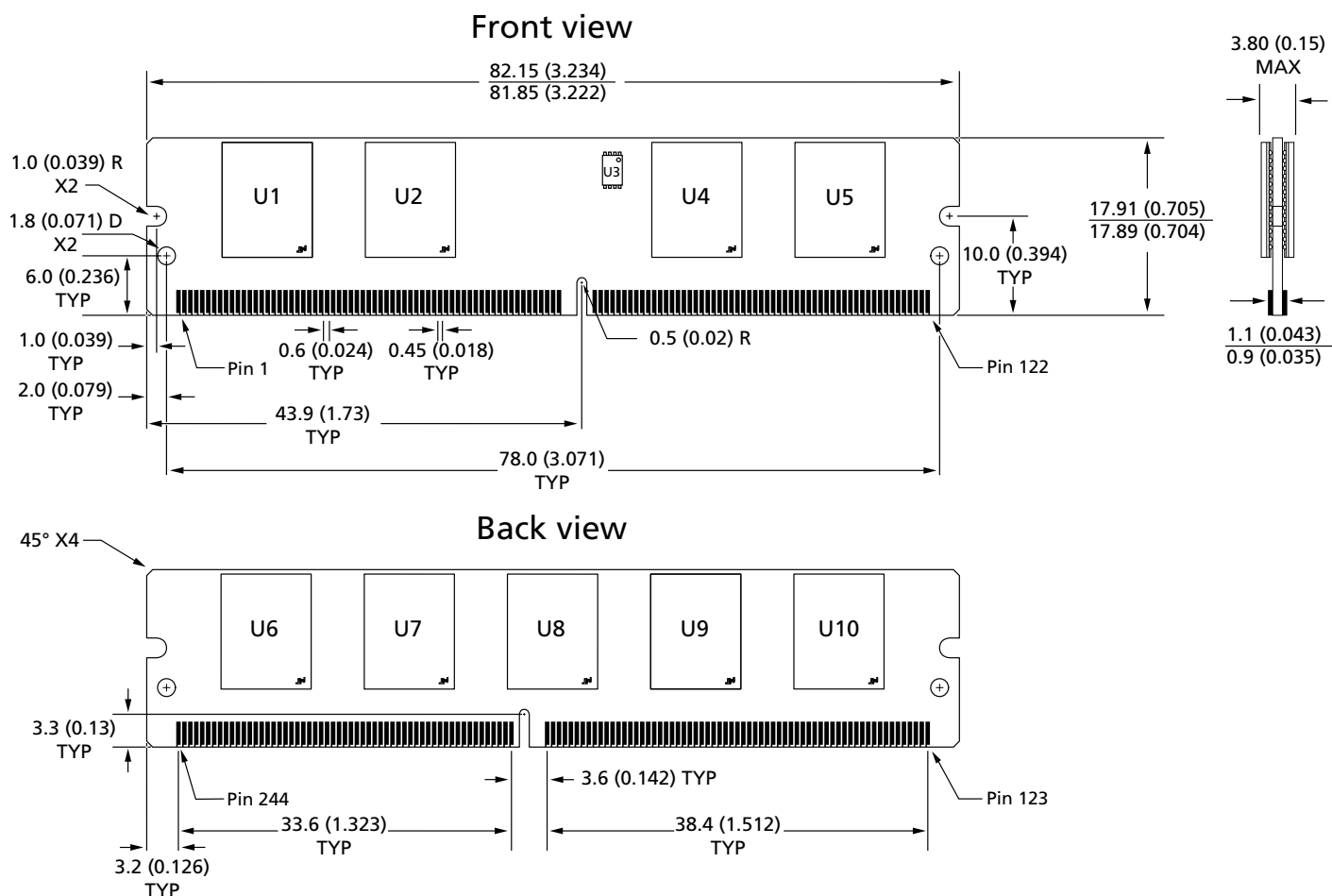
Figure 3: 244-Pin DDR3 ULP Mini-UDIMM
