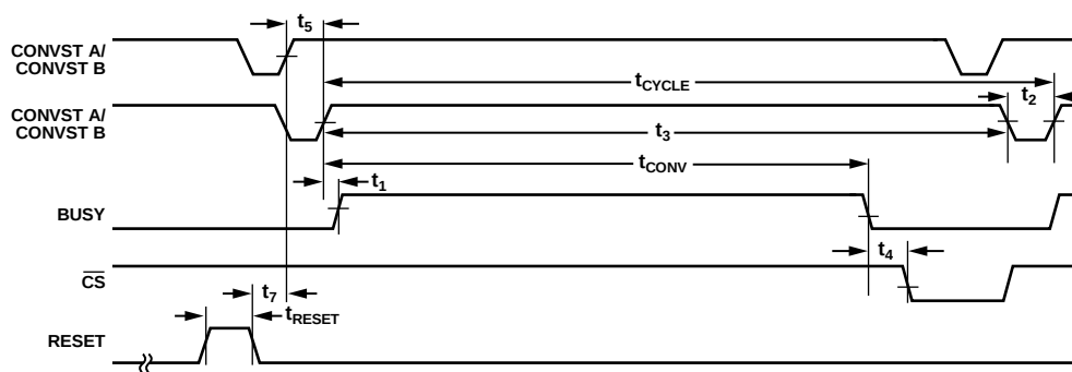
Figure 2. CONVST x Timing—Reading After a Conversion
