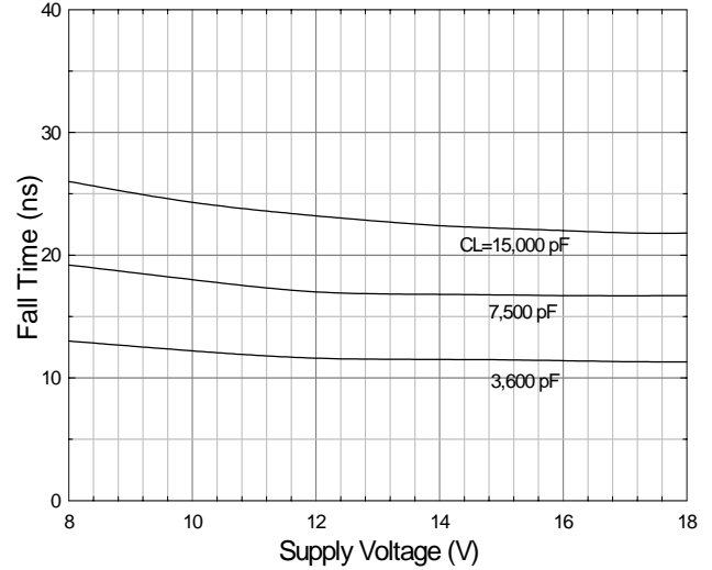
Fig. 6 Fall Time vs. Supply Voltage
