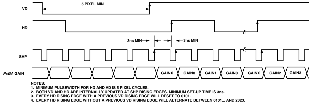
Figure 9. PxGA Mode 1 (Mosaic Separate) Detailed Timing
