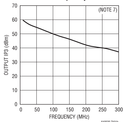
Equivalent Output IP3 vs Frequency
