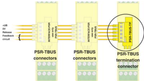
Connection diagram
