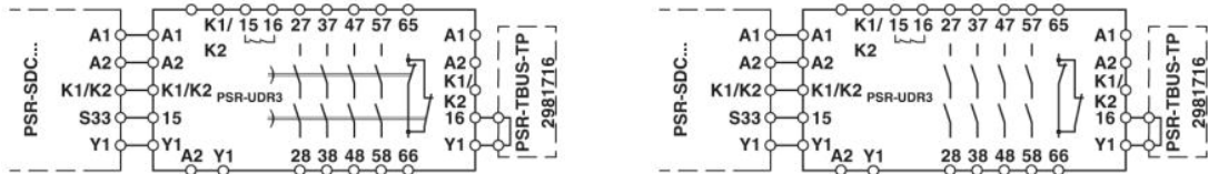
Circuit diagram
