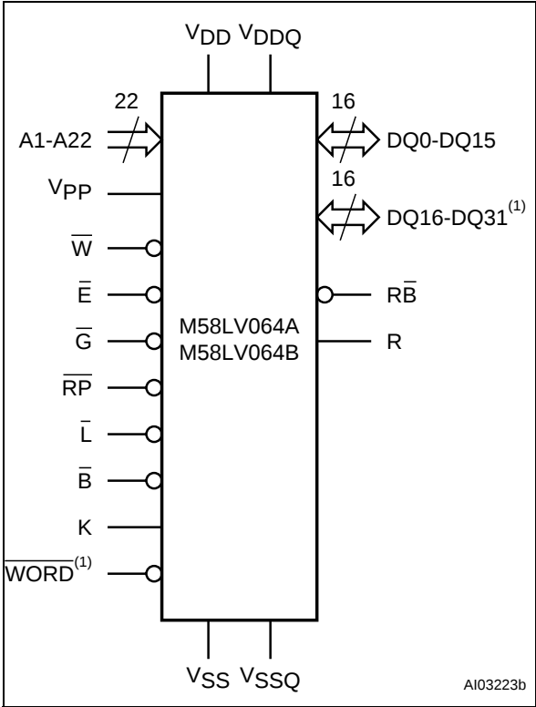
Figure 2. Logic Diagram
