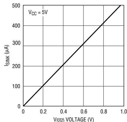
LTC1296 SS0 Sink Current vs V SS0
