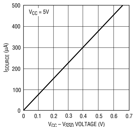
LTC1296 SS0 Source Current vs V CC - V SS0
