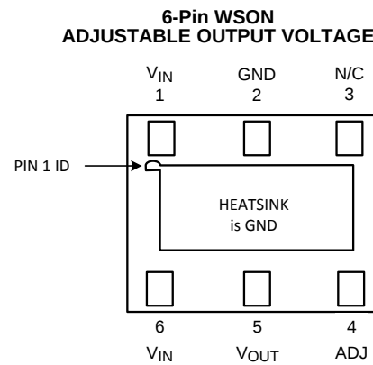
Figure 2. Bottom View
