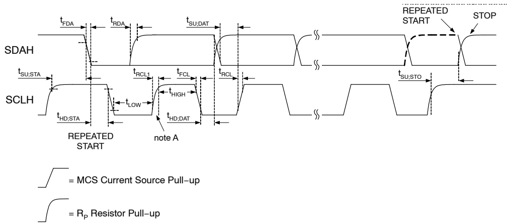
Figure 4. I²C Interface Timing for High-Speed Mode
