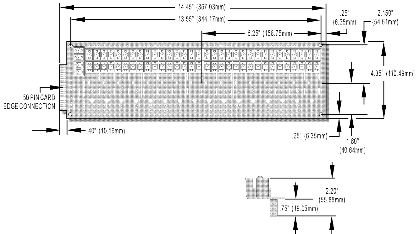
PB16C DIMENSIONS
