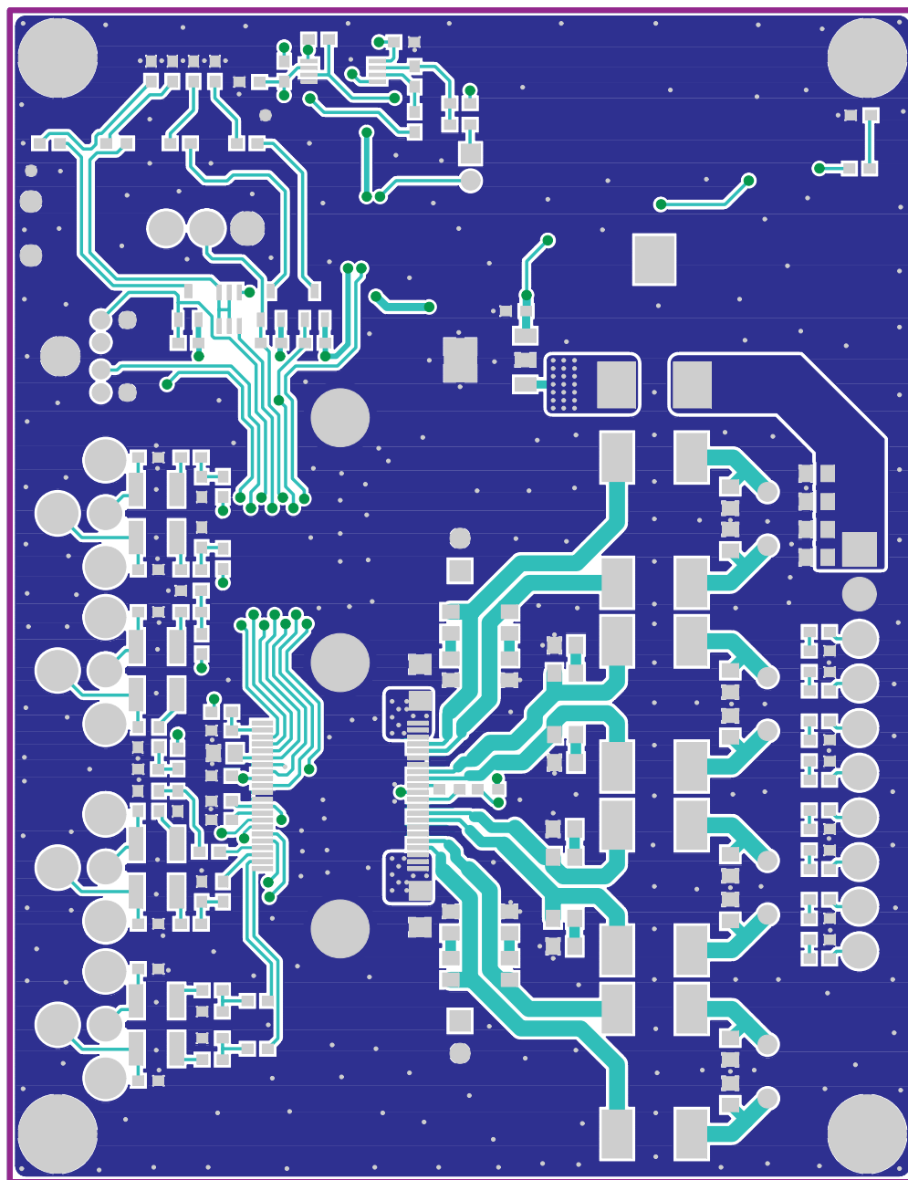
Figure 1-13. TAS5424AEVM3 Top Copper Layer
