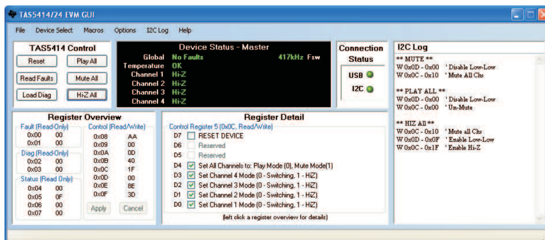
Figure 1-2. Main Window
