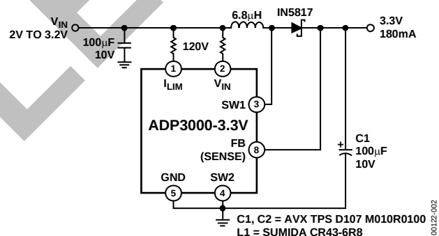
Figure 2. Typical Application
