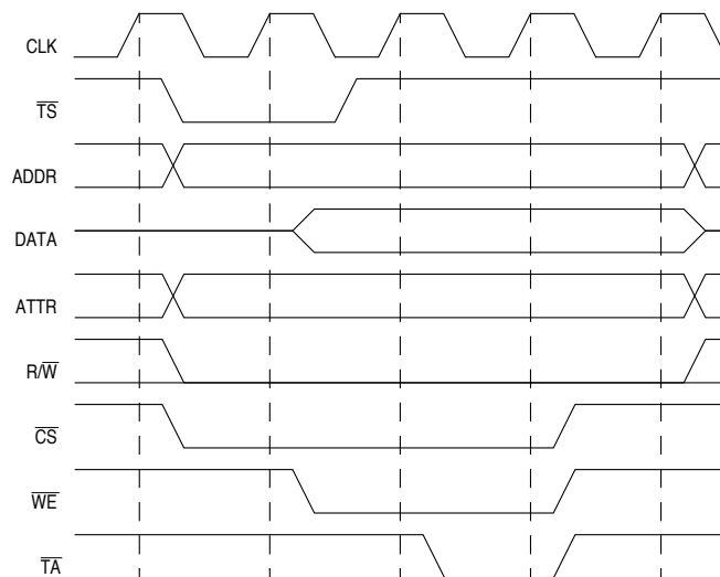
Figure 8-14. Address Hold Timing with WRAH = 1
