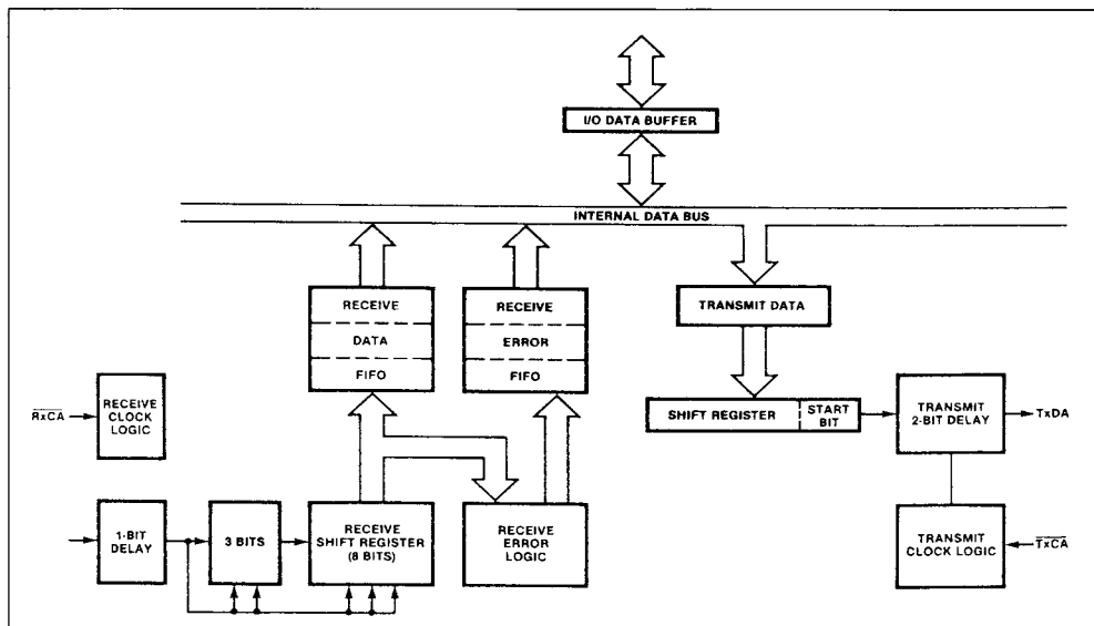
Figure 4 : Data Path.
