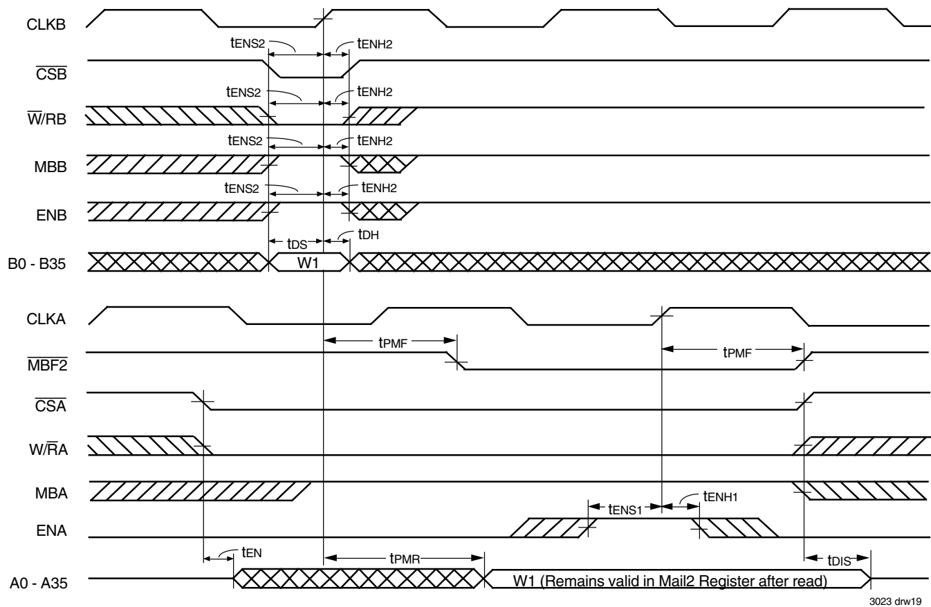
Figure 16. Timing for \overline{\text{Mail2}} Register and \overline{\text{MBF2}} Flag
