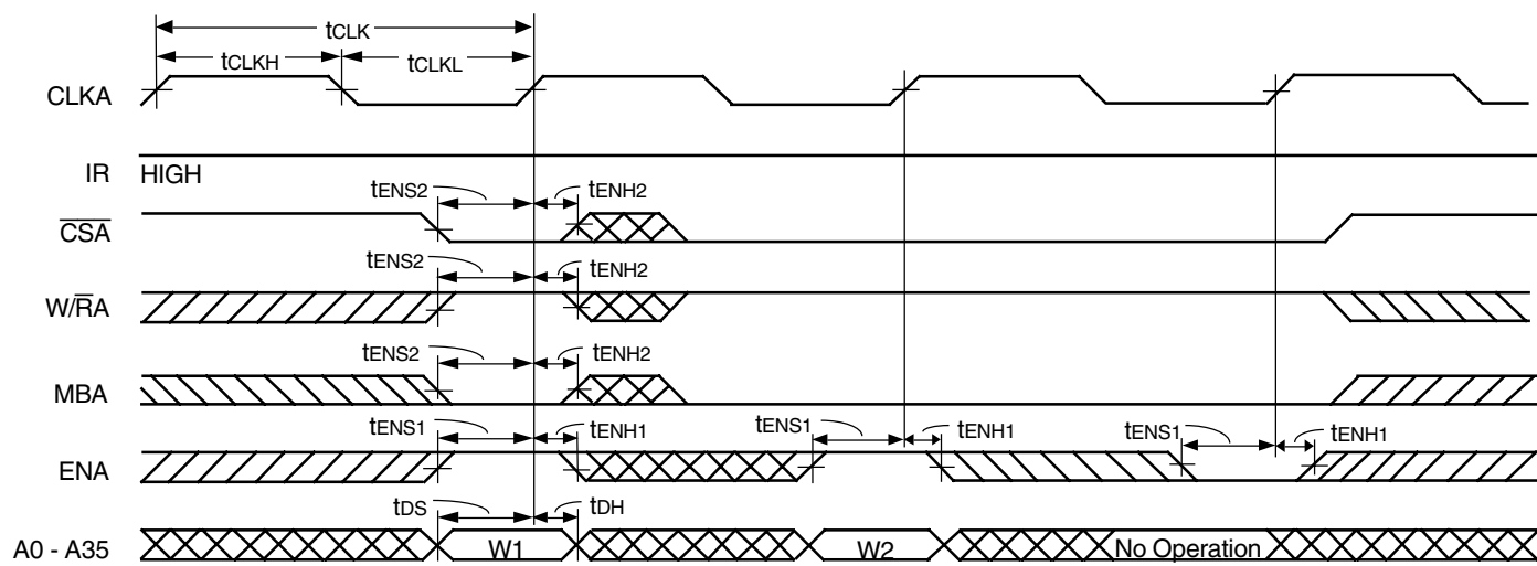
Figure 5. FIFO Write Cycle Timing
