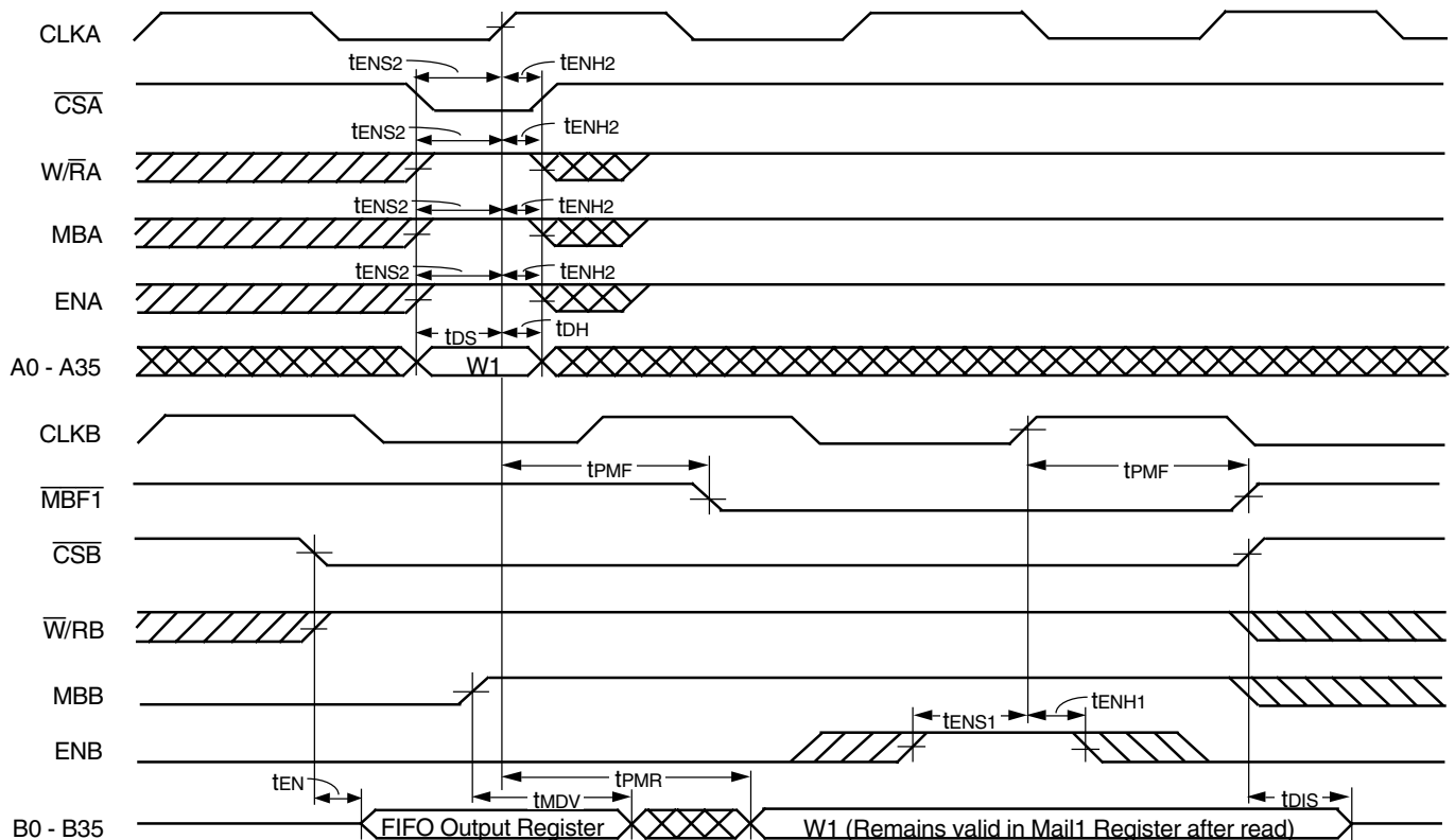
Figure 15. Timing for Mail1 Register and MBF1 Flag
