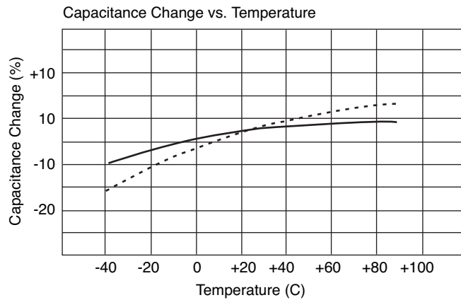
Temperature Characteristics
