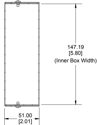
SECTION A-A End View of Assembly
