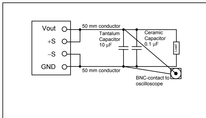
Output ripple and noise test set-up. Additional C_O = 470 µF was added close to the output pins.
