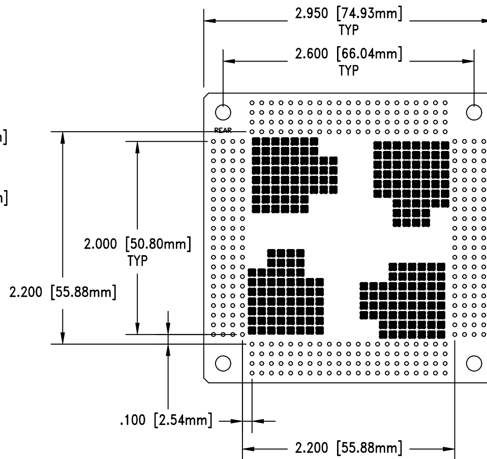
BOTTOM VIEW
