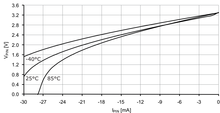
Figure 37-196. I/O pin output voltage vs. source current.
