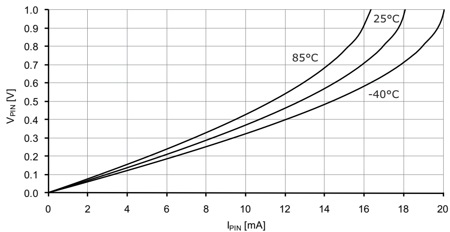
Figure 37-198. I/O pin output voltage vs. sink current.
