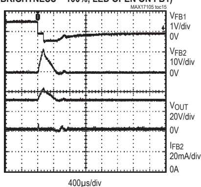
LED-OPEN FAULT PROTECTION (BRIGHTNESS = 100%, LED OPEN ON FB1)
