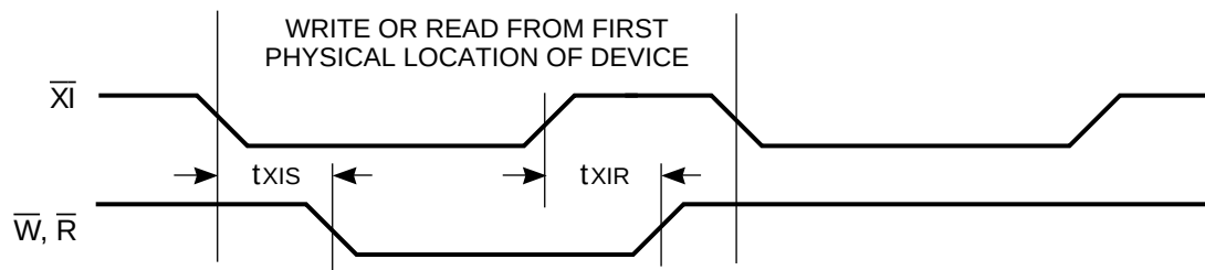
FIGURE 13. EXPANSION-IN TIMING
