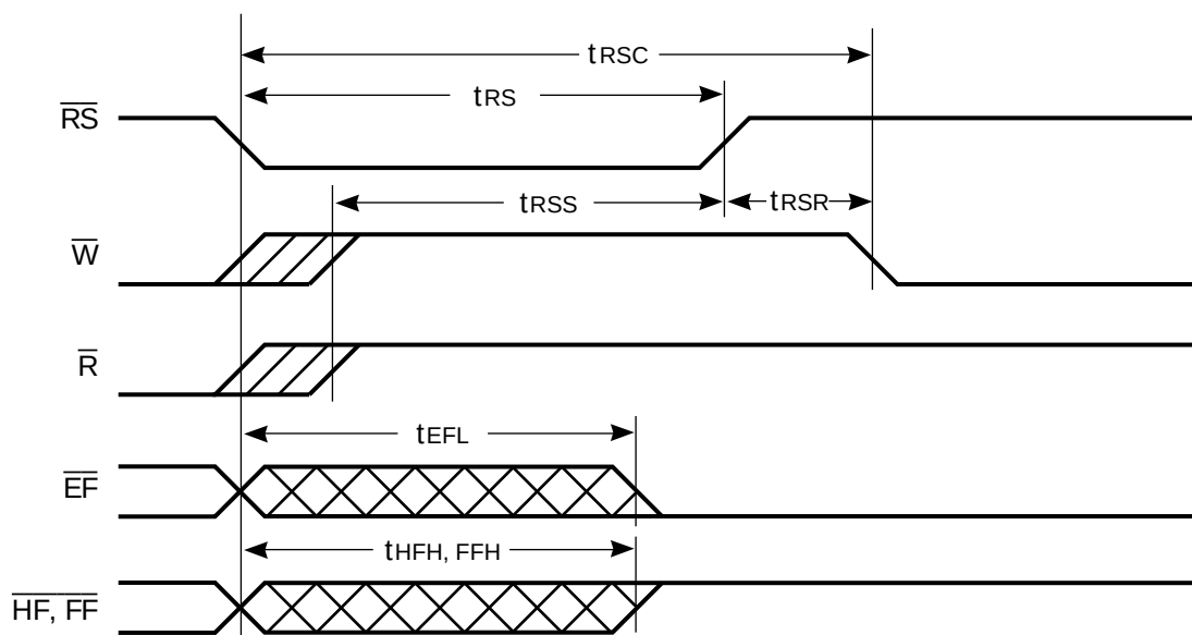
FIGURE 5. RESET TIMING
