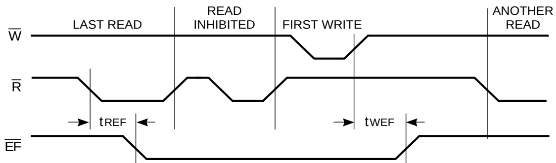
FIGURE 8. EMPTY FLAG BEHAVIOR FROM LAST READ TO FIRST WRITE
