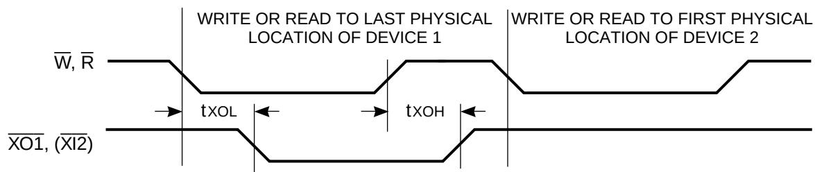
FIGURE 12. EXPANSION-OUT TIMING
