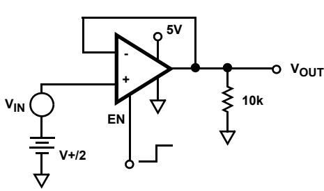
FIGURE 29. TEST CIRCUIT FOR A_V = +1
