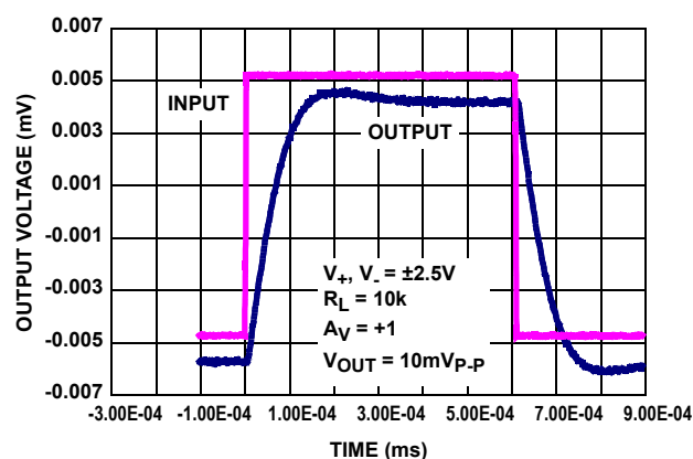
FIGURE 7. SMALL SIGNAL TRANSIENT RESPONSE
