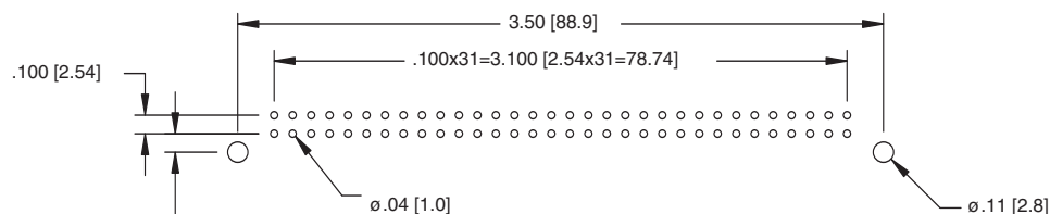
Recommended PCB Layout - Female
