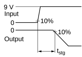
Response Waveform
