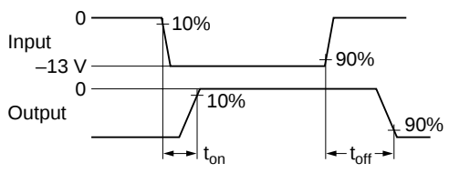
Response Waveform
