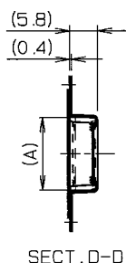
SECT. D-D
