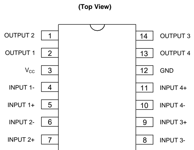
(DIP-14/ P Package)
