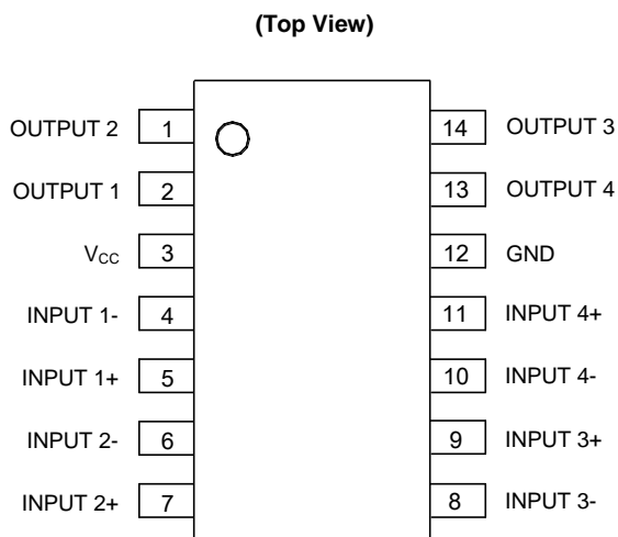
(SOIC-14/ M Package / TSSOP-14/ G Package)
