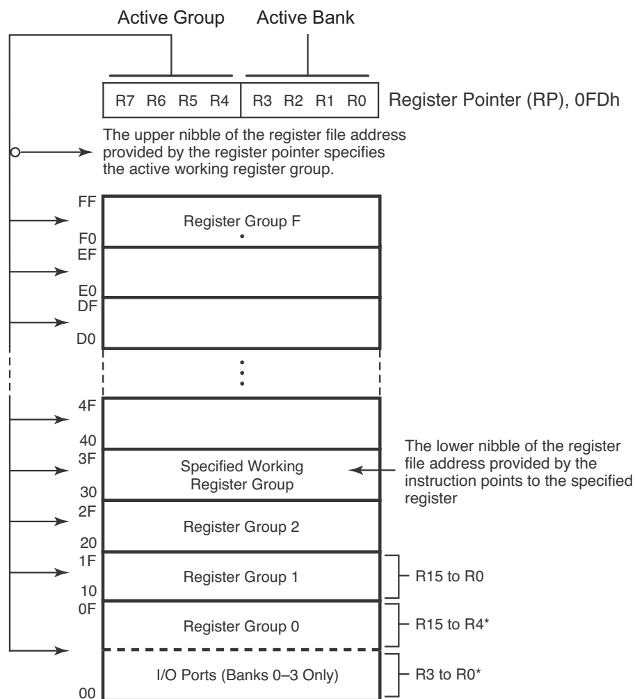
Figure 10. Register Pointer—Detail
