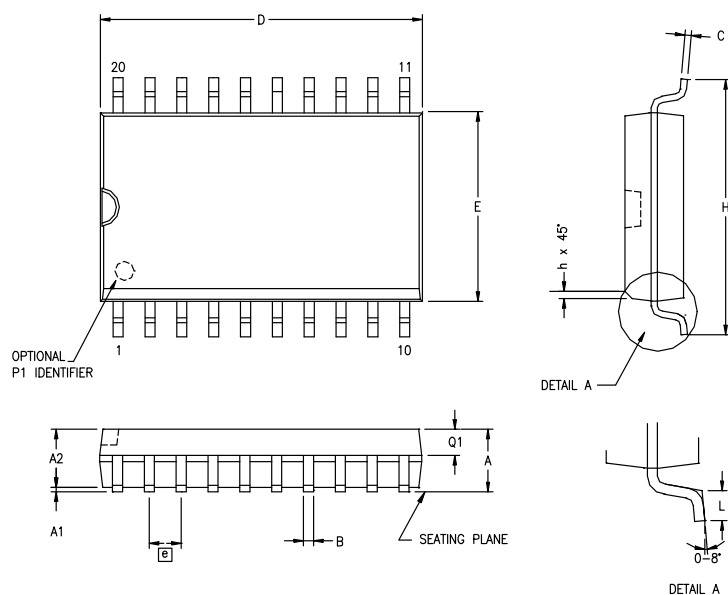
Figure 45. 20-Pin SOIC Package Diagram
