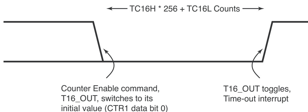
Figure 27. T16_OUT in SINGLE-PASS Mode
