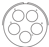
LAYOUT # OF CONTACTS 32-63 5-#4 SERIES ▼ SERVICE RATING D
