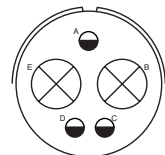
LAYOUT # OF CONTACTS 32-1 3-#12; 2-#0 SERIES ⊕ ⊙ ▼ SERVICE RATING E(A); D(All others)
