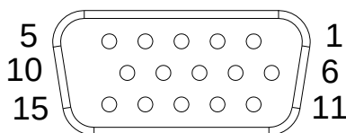
Figure 2.8 VGA Connector
