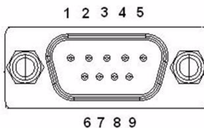
Figure 2.11 COM Port Connector
