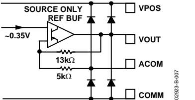
Figure 7. Circuit E
