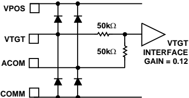
Figure 5. Circuit C
