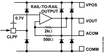
Figure 6. Circuit D
