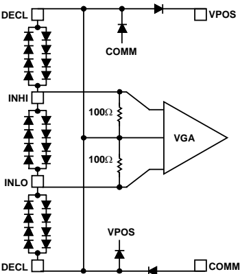
Figure 3. Circuit A
