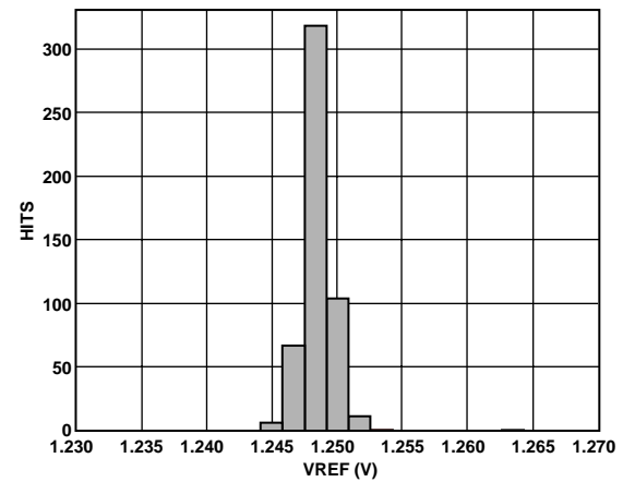
Figure 37. VREF Distribution
