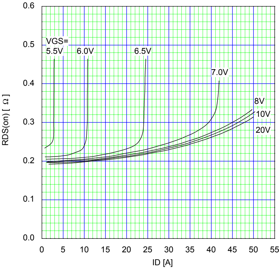
Typical Drain-Source on-state Resistance R_{DS(on)}=f(I_D):80\text{ }\mu\text{s pulse test}, T_{ch}=25^\circ\text{C}
