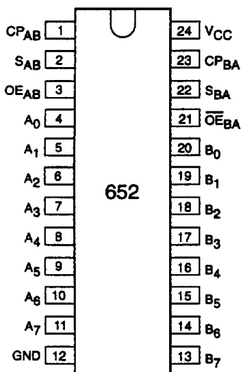
Fig.1 Pin configuration.
