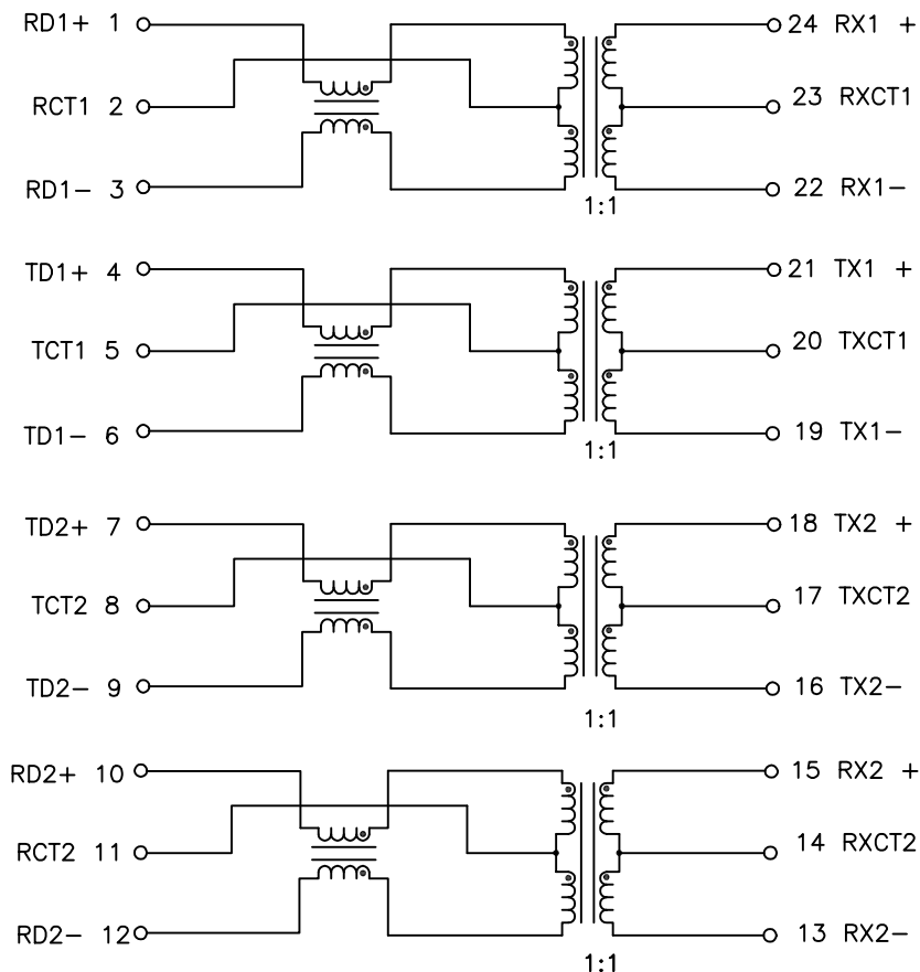
SCHEMATIC
