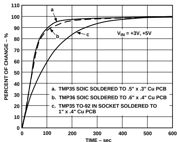
Figure 13. Thermal Response Time in Still Air
