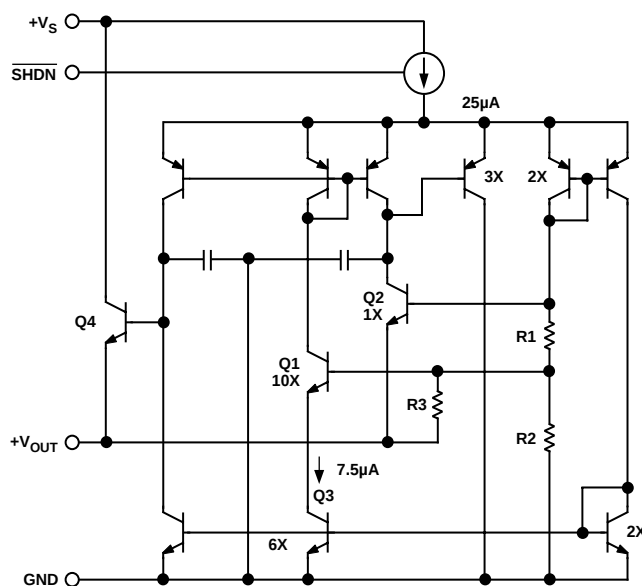
Figure 1. Temperature Sensor Simplified Equivalent Circuit
