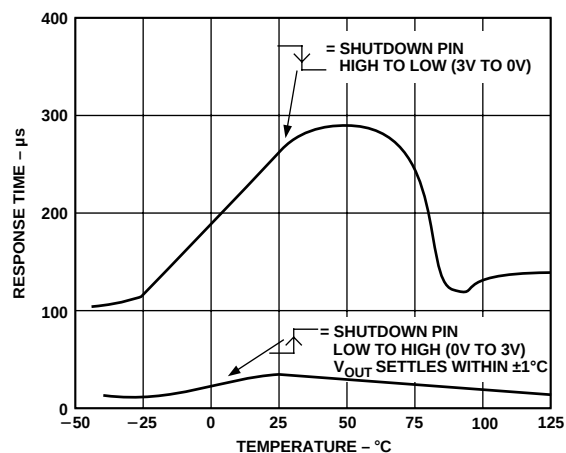
Figure 11. V_{OUT} Response Time for Shutdown Pin vs. Temperature
