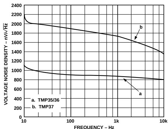
Figure 17. Voltage Noise Spectral Density vs. Frequency
