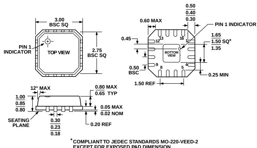
Figure 51. 16-Lead Lead Frame Chip Scale Package [LFCSP] 3 mm × 3 mm Body (CP-16-3) Dimensions in millimeters
