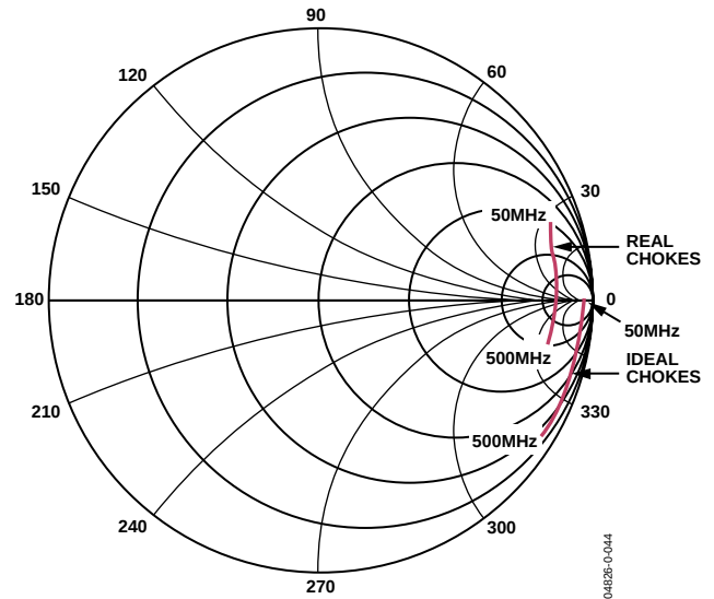
Figure 41. IF Port Loading Effects due to Finite-Q Pull-Up Inductors (Murata BLM18HD6015N1D Chokes)
