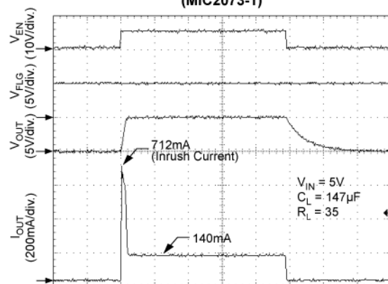
Turn-On/Turn-Off (MIC2073-1)
