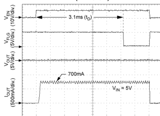
Enabled Into Short (MIC2073-1)
