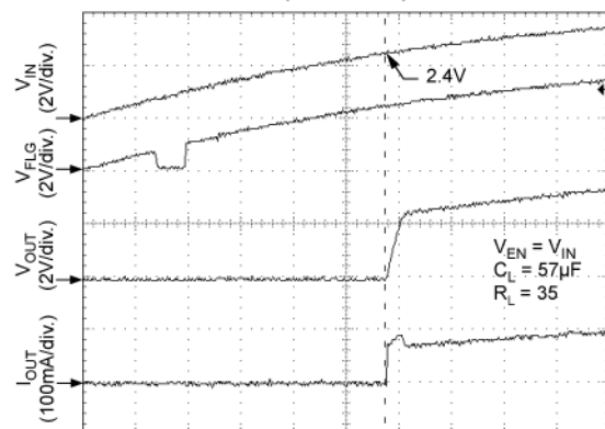
UVLO— V_{IN} Rising (MIC2073-1)
