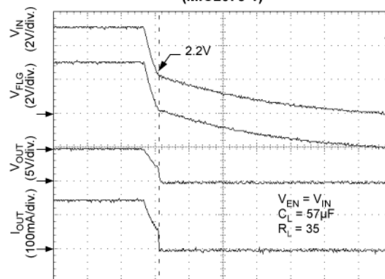
UVLO— V_{IN} Falling (MIC2073-1)
