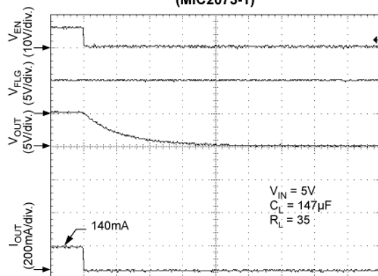
Turn-Off (MIC2073-1)
